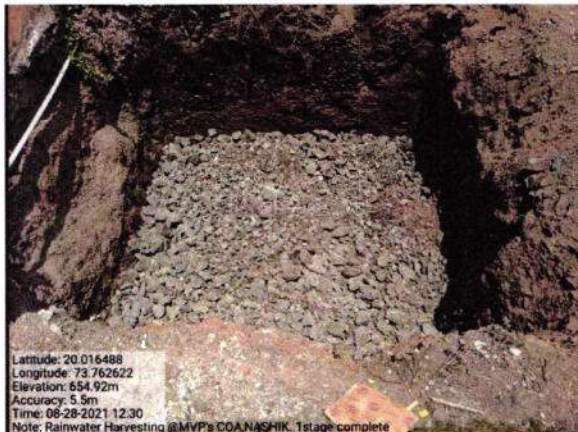
Rain water harvesting pit 1 (Terrace rain water) refilling with granular material
