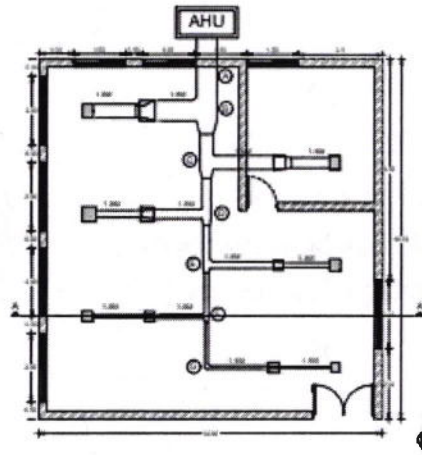
DUCTING LAYOUT
