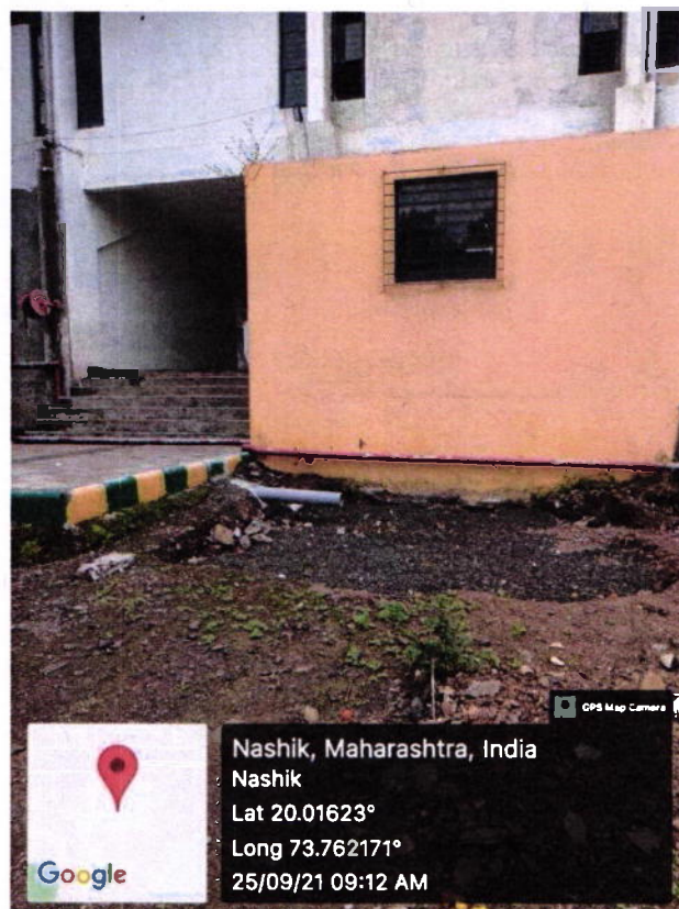
Rain water harvesting pit 1 (Terrace rain water) refilling with granular material Terrace storm water pipe connected to pit
